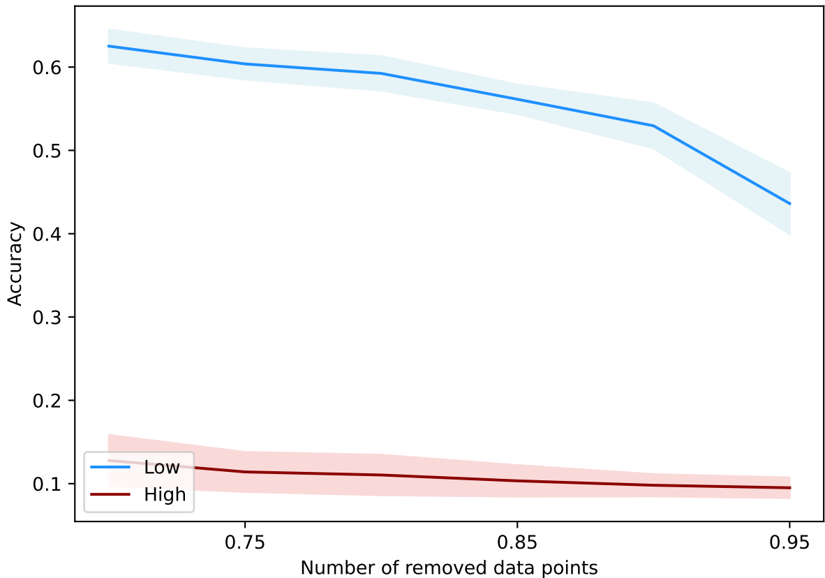
DataAttrOpt(10000, 0.1, 15, best, +b, alpha=best) - cifar10-embedding
